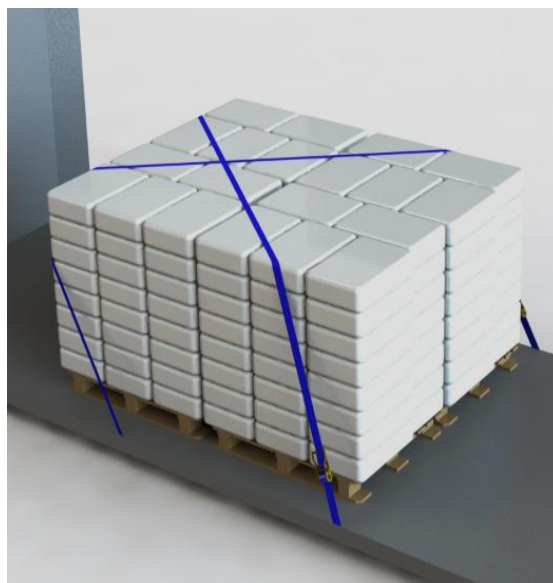
Figure 3: Four pallets with cross spring lashing
