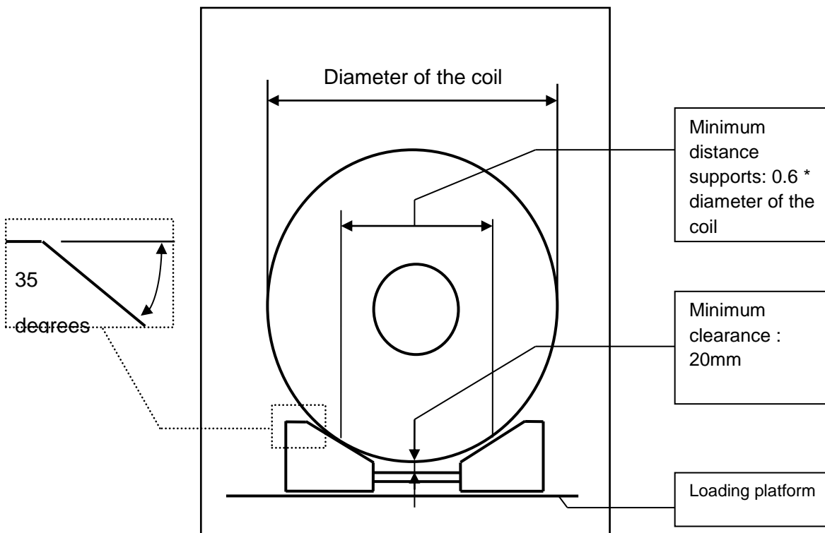
Characteristics of a wedge bed
