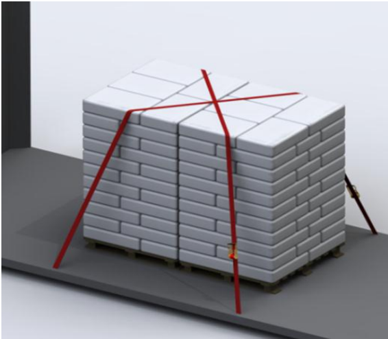
Figure 1: Two pallets with cross lashing
