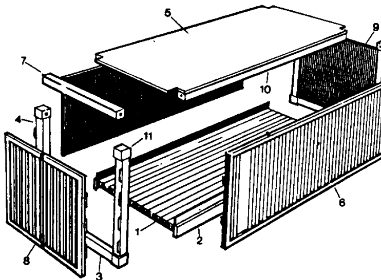
Picture 1 Exploded view of the design and construction of the container
