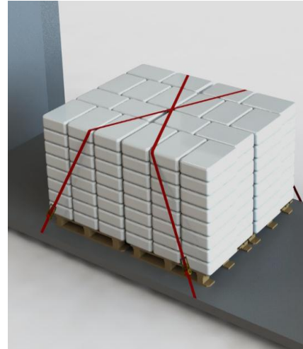
Figure 2: Four pallets with cross lashing
