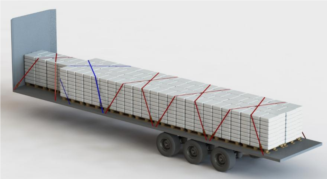
Figure 4: Trailer with a combination of blocking, cross top- and spring lashing
