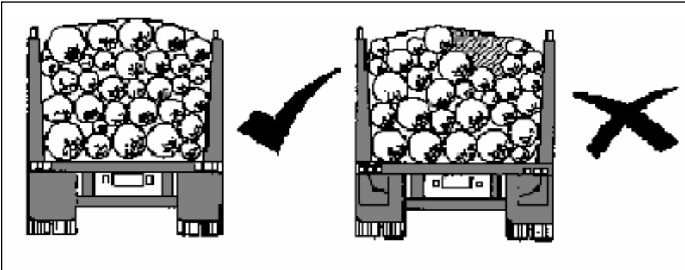
Correct (left) and incorrect (right) loading of round timber
