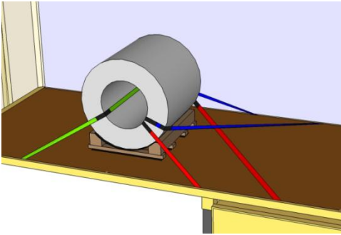
Figure x Low coil weight
